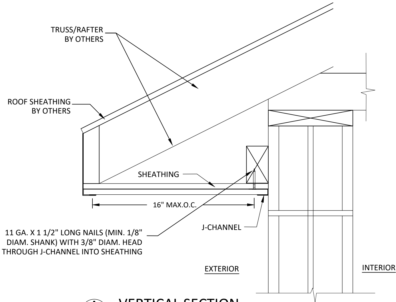
A 3 VERTICAL SECTION SOFFIT INSTALLATION DETAIL BUILDERS TRIPLE 4 SINGLE SPAN
