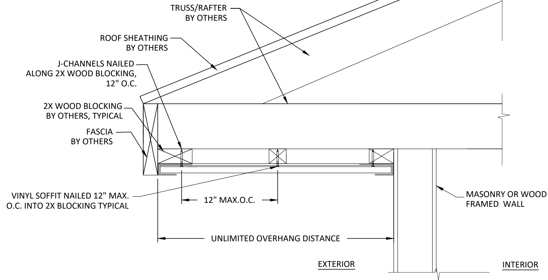
A 2 VERTICAL SECTION SOFFIT INSTALLATION DETAIL 2X WOOD FRAMING, TYP.
